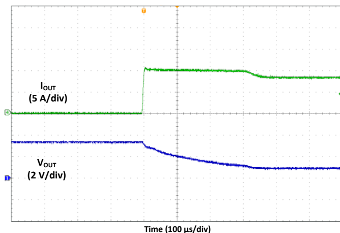
Fig. 36 Over-current Limiting
