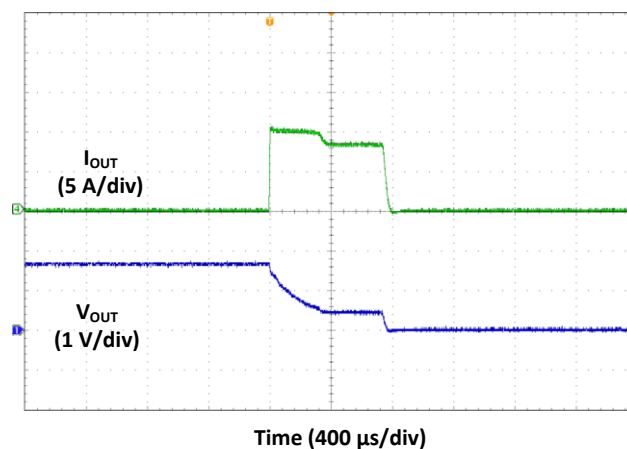
Fig. 37 Hiccup Mode Current Limit Shut-down
